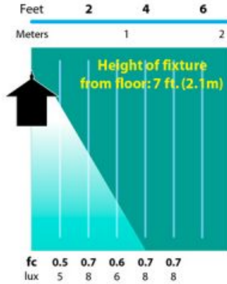
Half Spread Photometrics 8 ft. (2.4m) diameter
