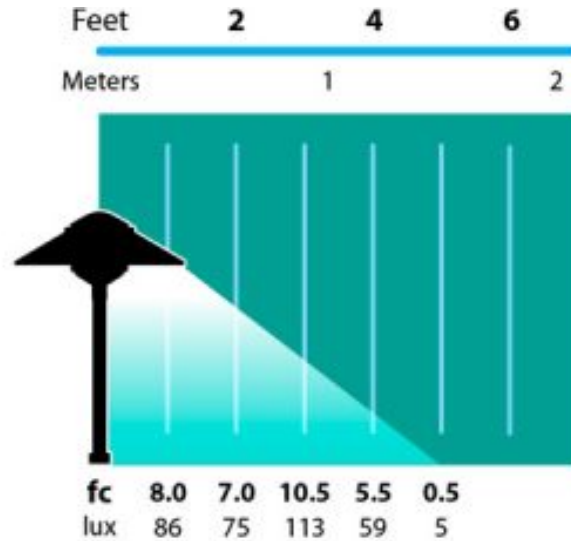
Half Spread Photometrics 10 ft. (3.0m) diameter
