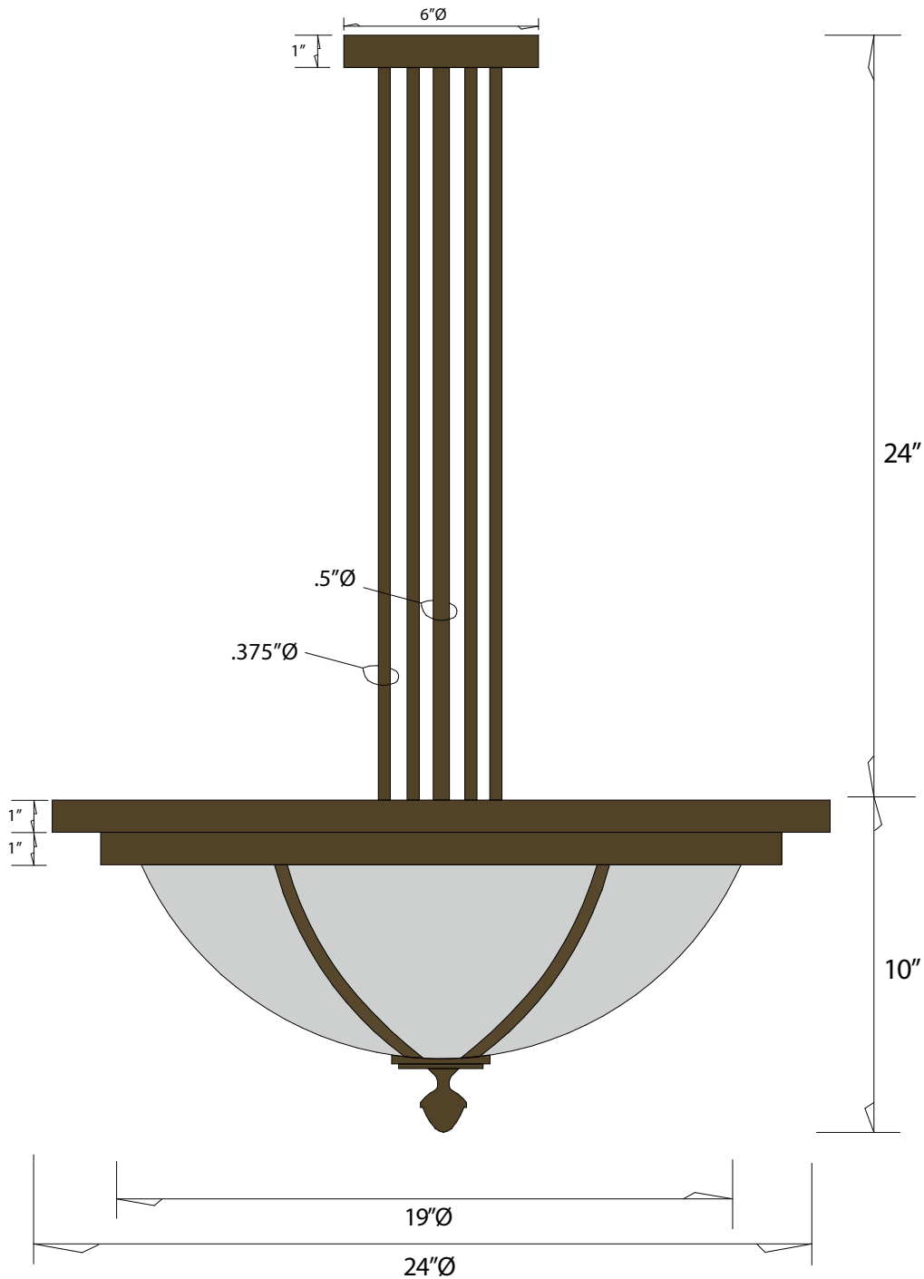
SIDE VIEW
